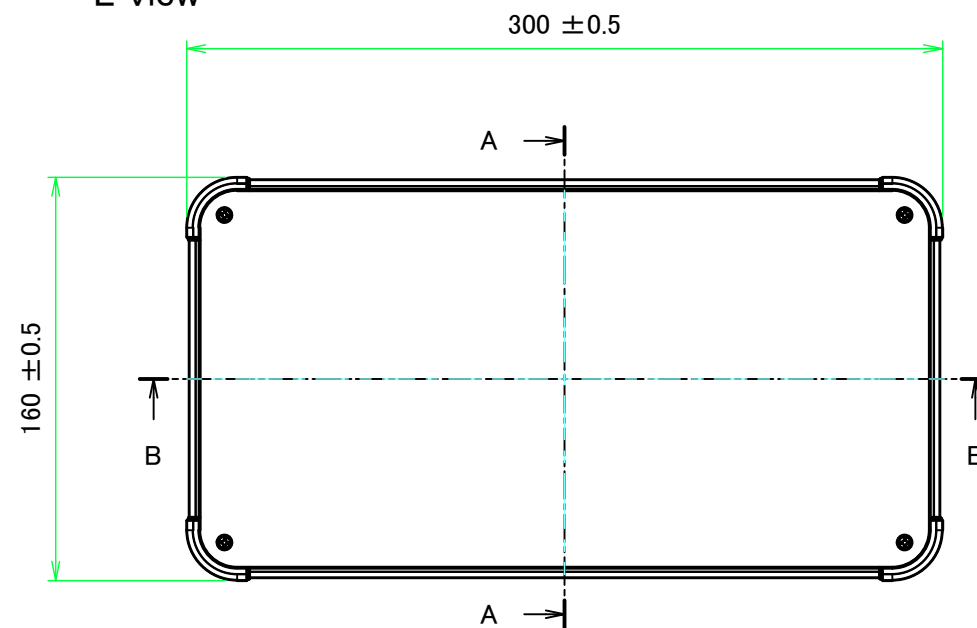
E view
